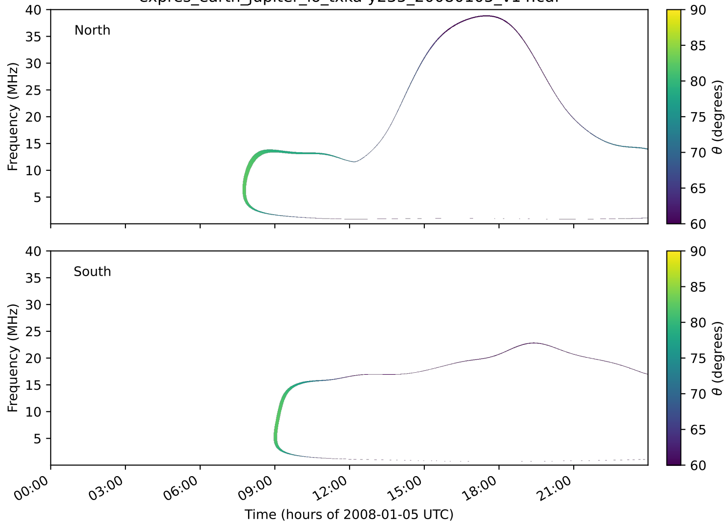
expres_earth_jupiter_io_txka-y235_20080105_v14.cdf
