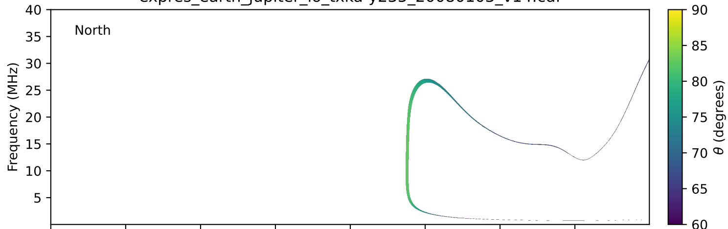
expres_earth_jupiter_io_txka-y235_20080103_v14.cdf
