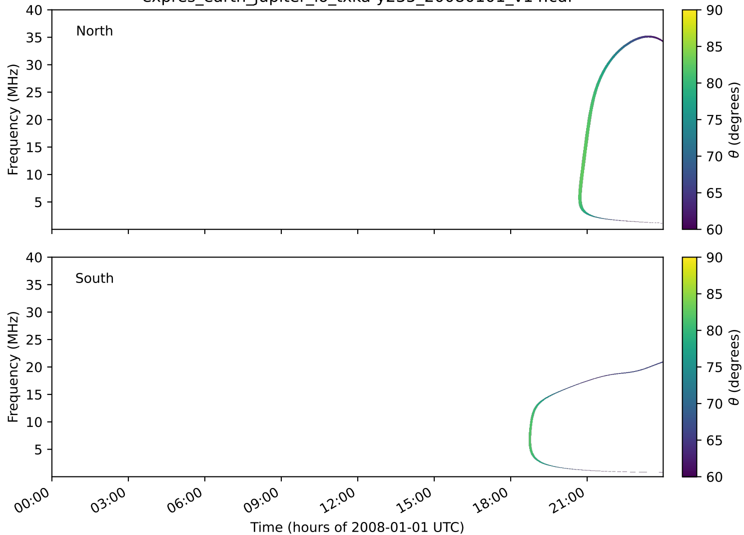
expres_earth_jupiter_io_txka-y235_20080101_v14.cdf
