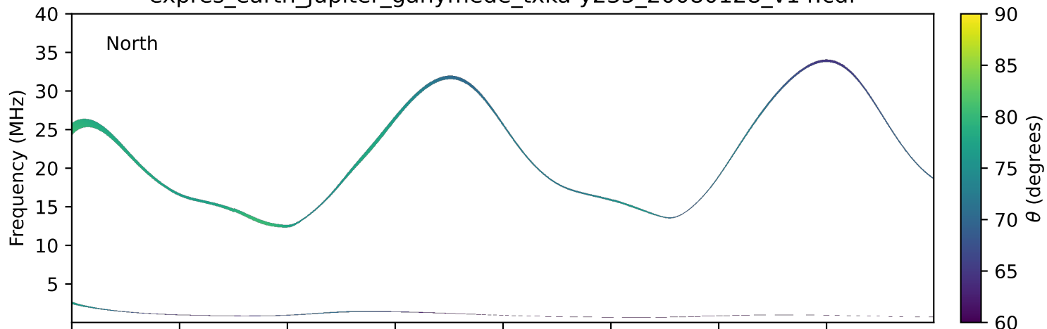
expres_earth_jupiter_ganymede_txka-y235_20080128_v14.cdf
