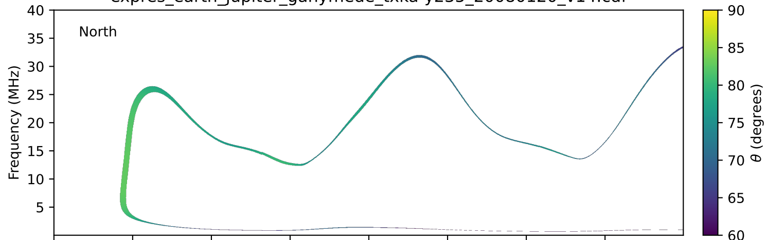
expres_earth_jupiter_ganymede_txka-y235_20080120_v14.cdf
