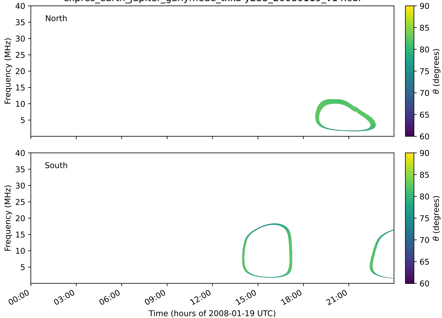
expres_earth_jupiter_ganymede_txka-y235_20080119_v14.cdf
