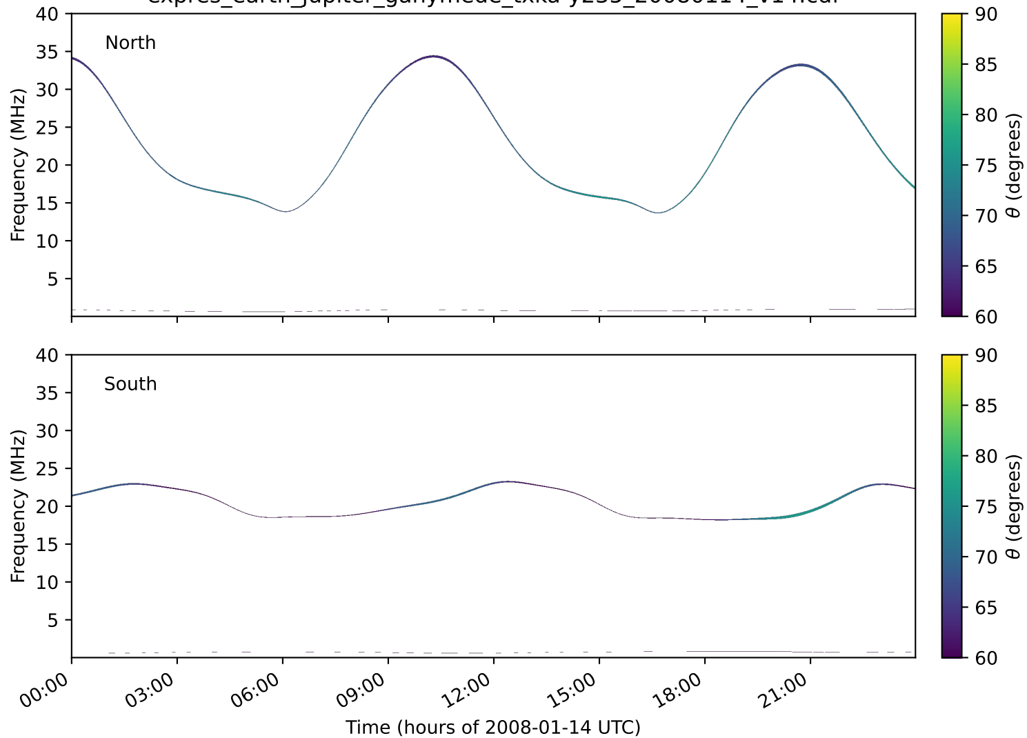
expres_earth_jupiter_ganymede_txka-y235_20080114_v14.cdf
