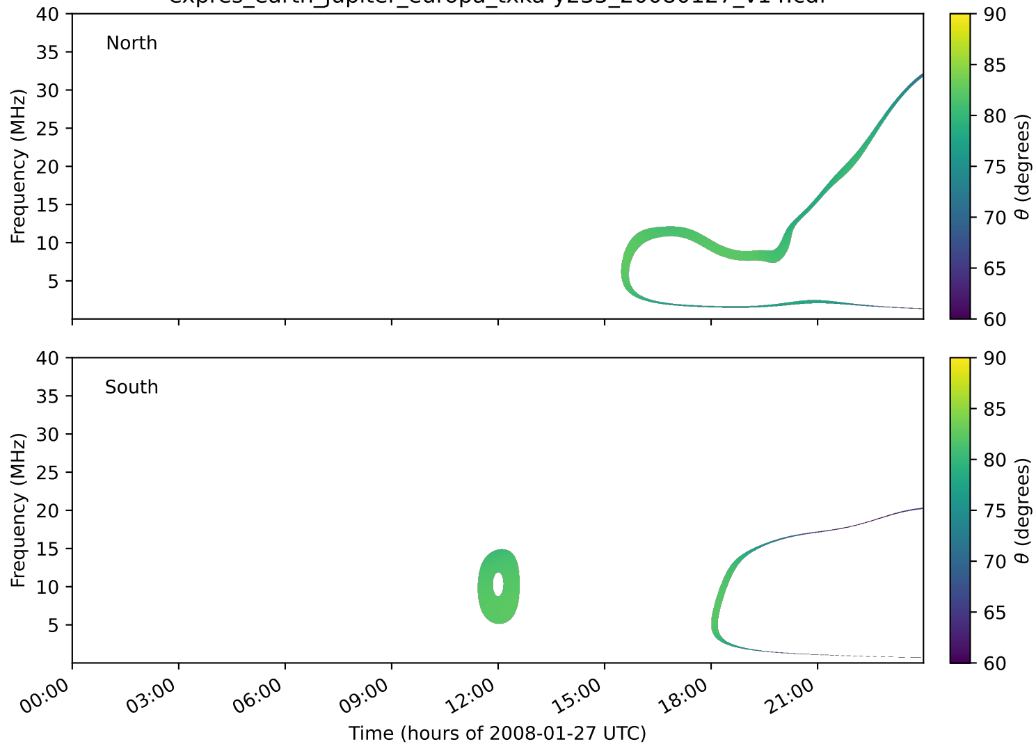
expres_earth_jupiter_europa_txka-y235_20080127_v14.cdf
