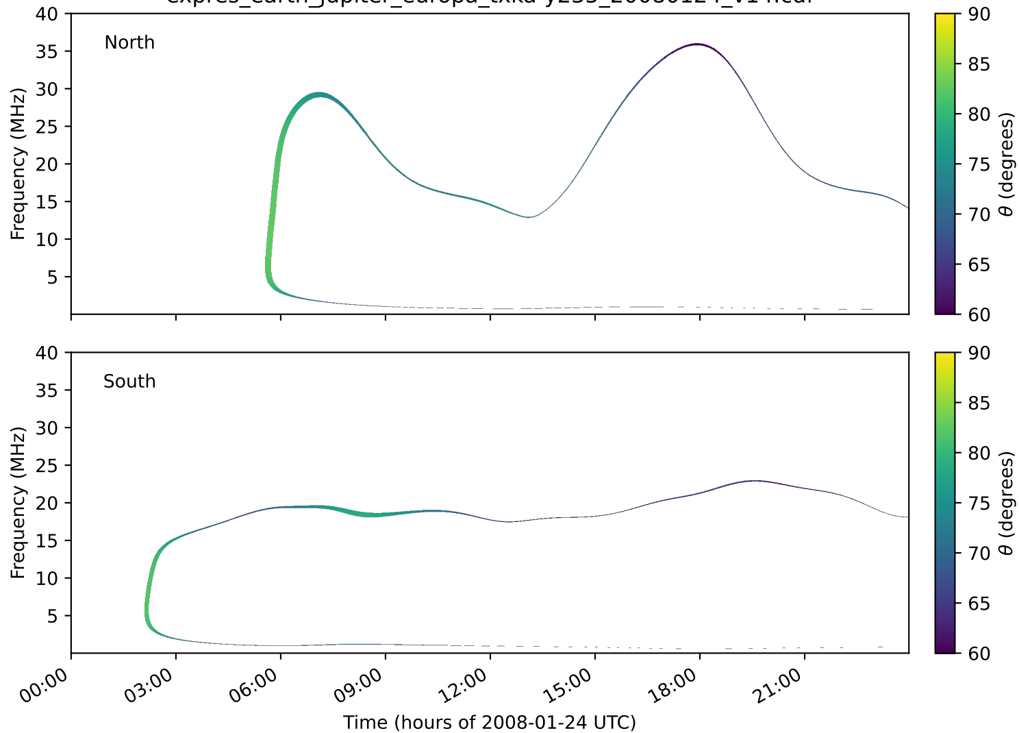
expres_earth_jupiter_europa_txka-y235_20080124_v14.cdf
