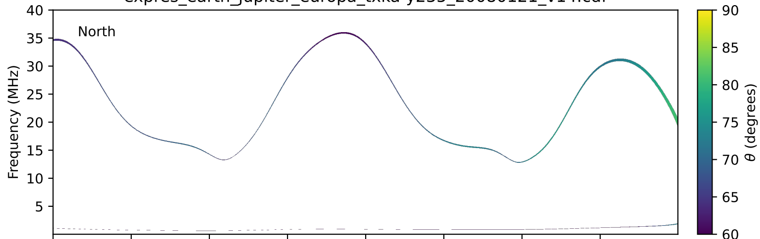
expres_earth_jupiter_europa_txka-y235_20080121_v14.cdf
