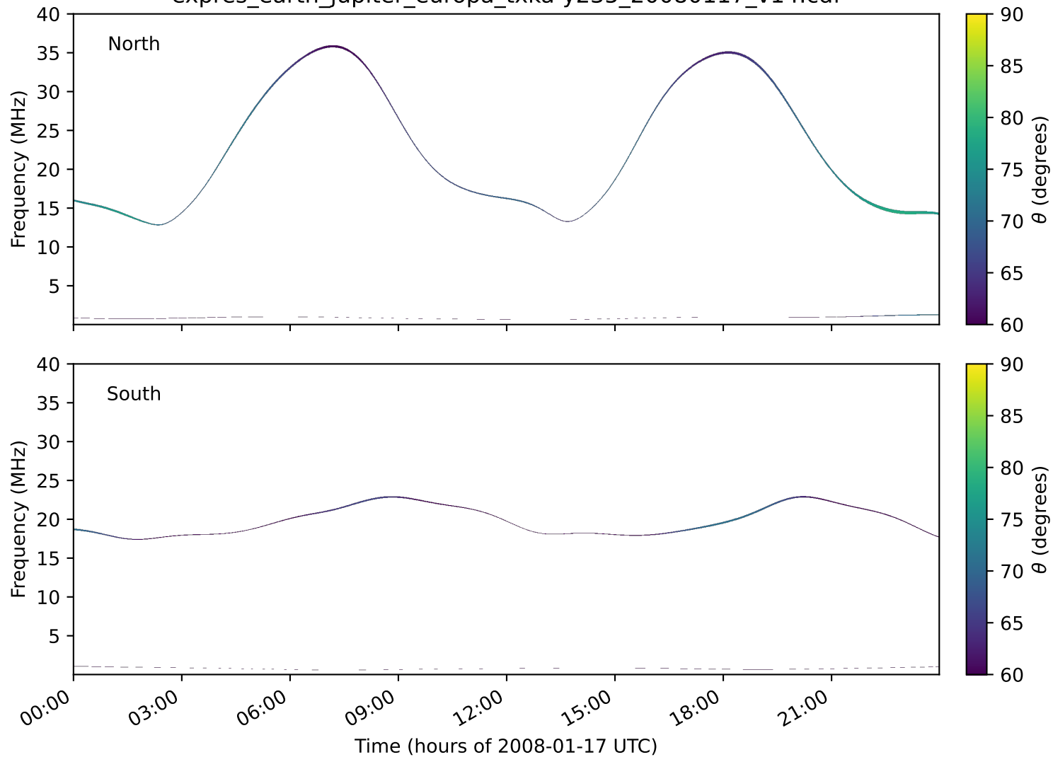
expres_earth_jupiter_europa_txka-y235_20080117_v14.cdf
