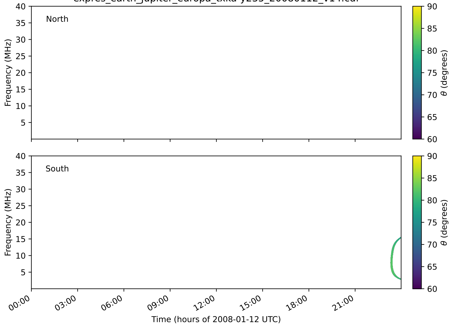
expres_earth_jupiter_europa_txka-y235_20080112_v14.cdf
