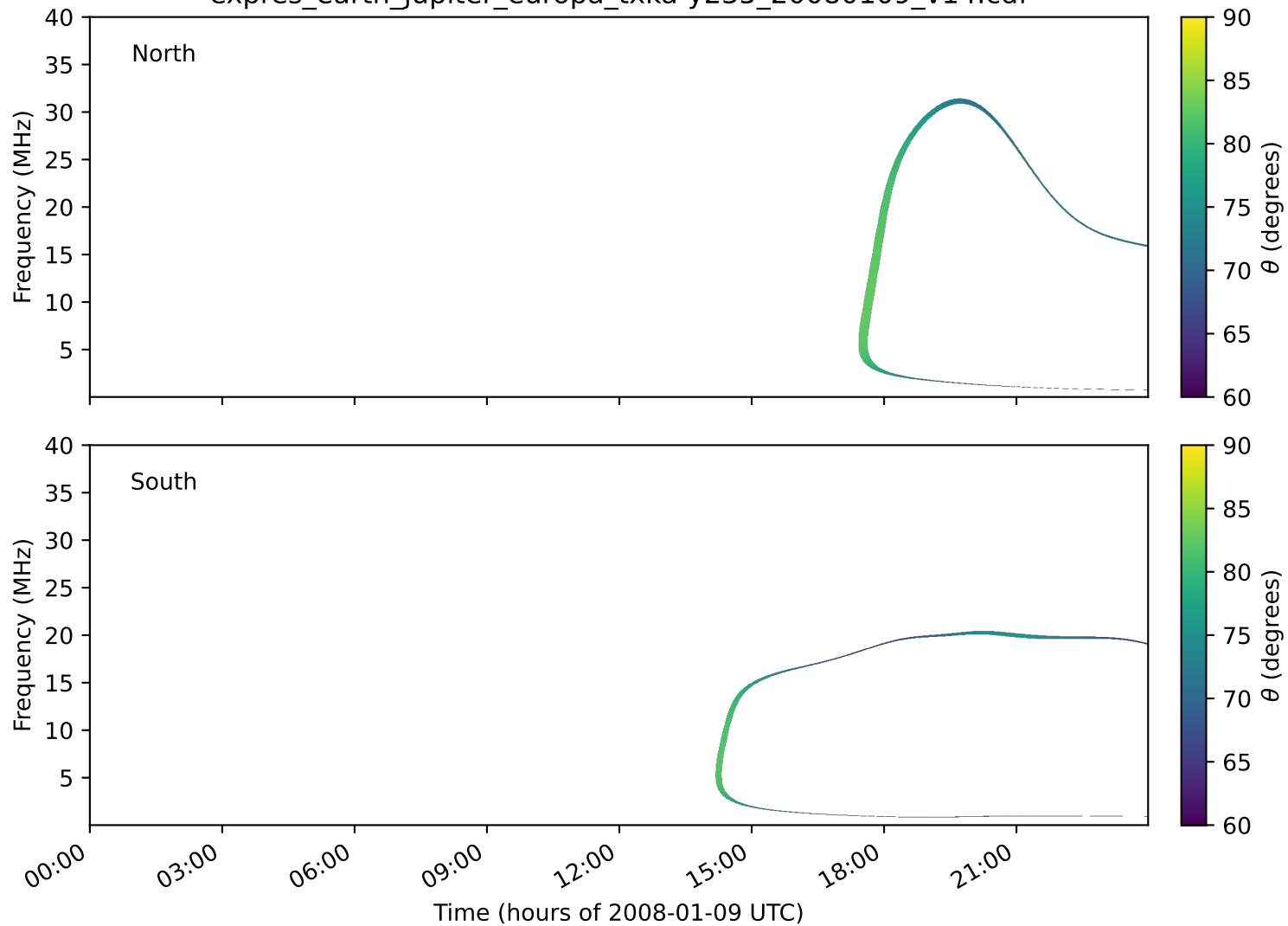
expres_earth_jupiter_europa_txka-y235_20080109_v14.cdf
