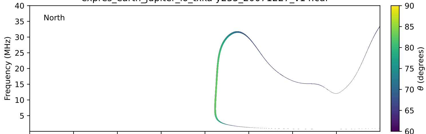
expres_earth_jupiter_io_txka-y235_20071227_v14.cdf
