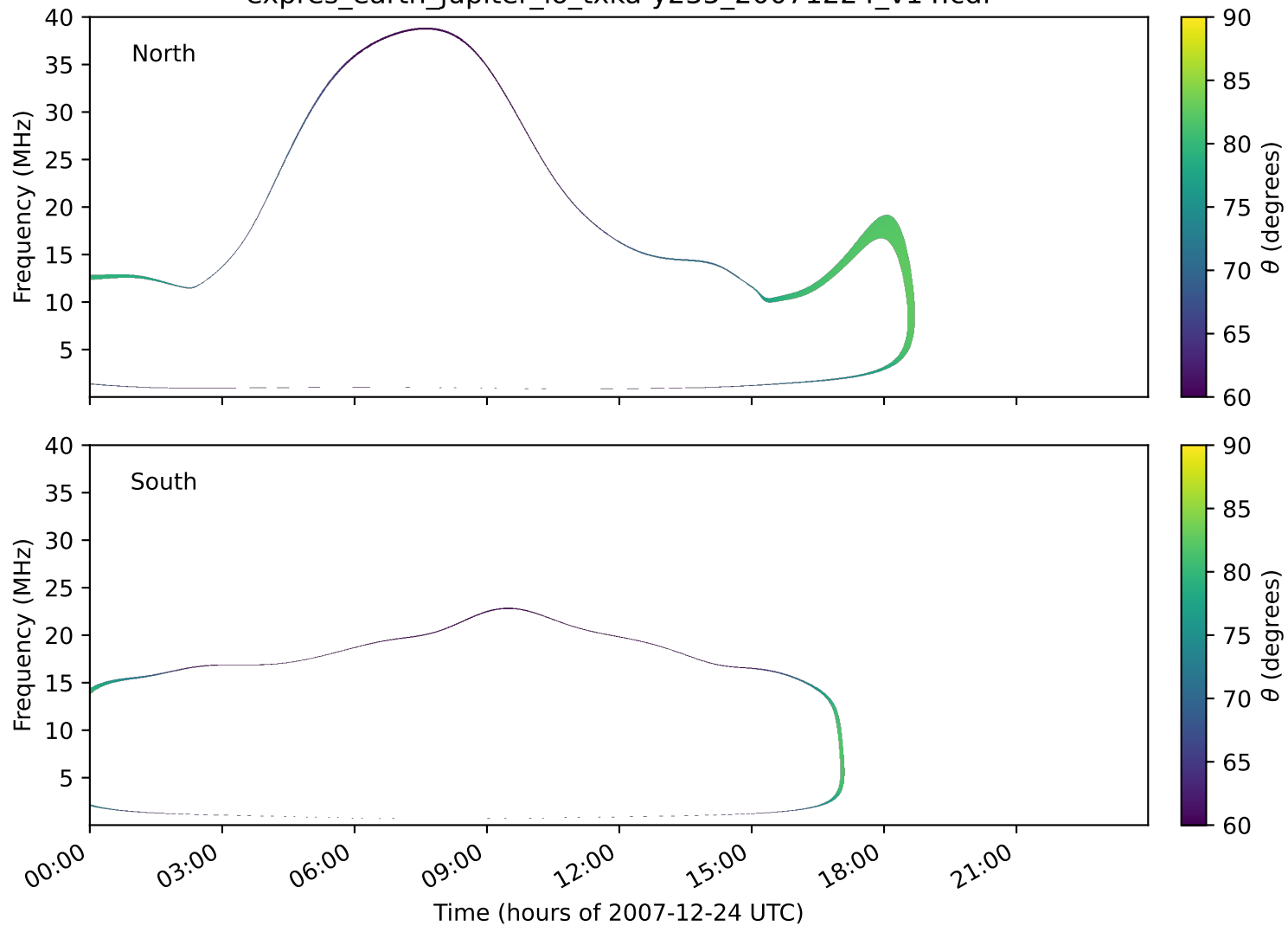
expres_earth_jupiter_io_txka-y235_20071224_v14.cdf
