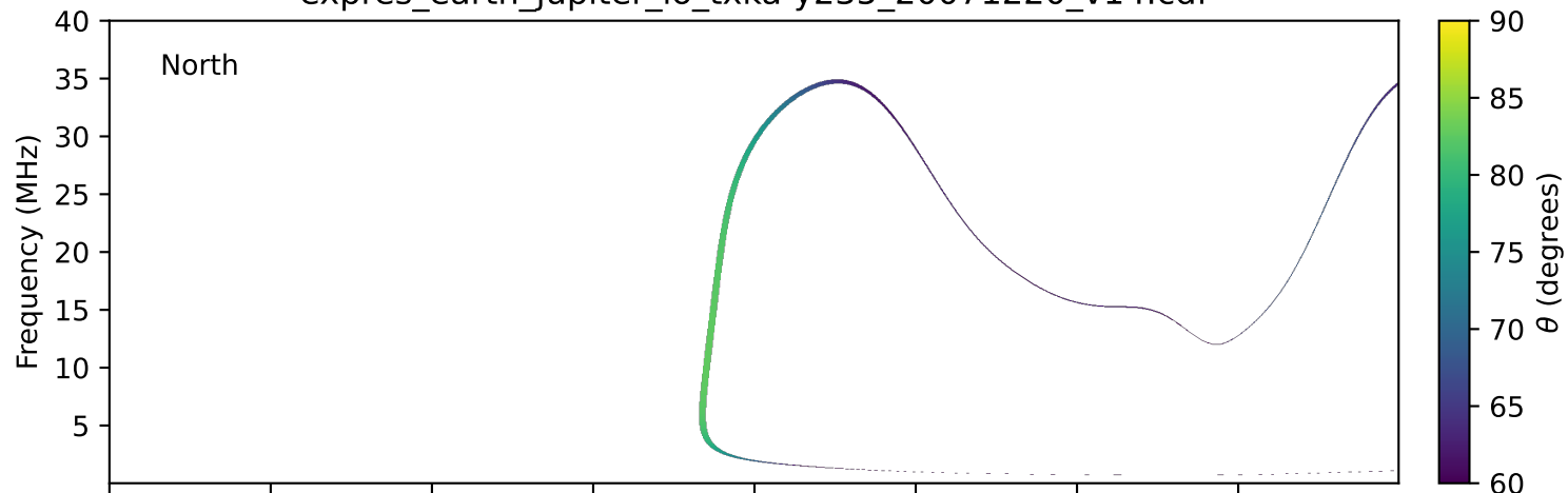
expres_earth_jupiter_io_txka-y235_20071220_v14.cdf
