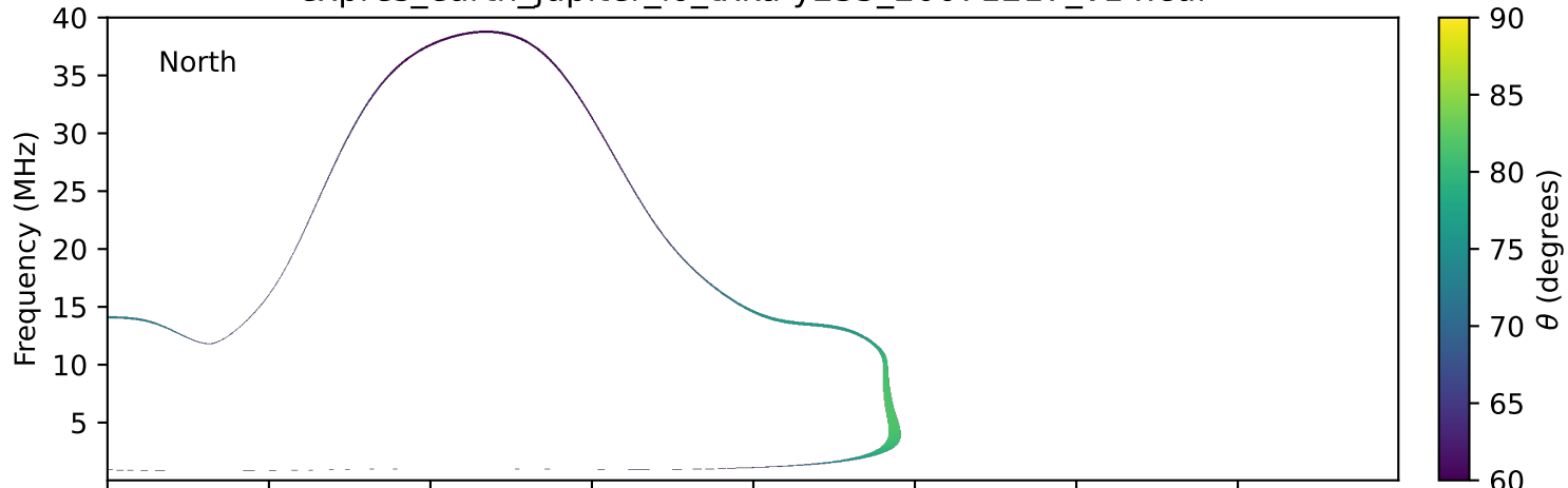
expres_earth_jupiter_io_txka-y235_20071217_v14.cdf
