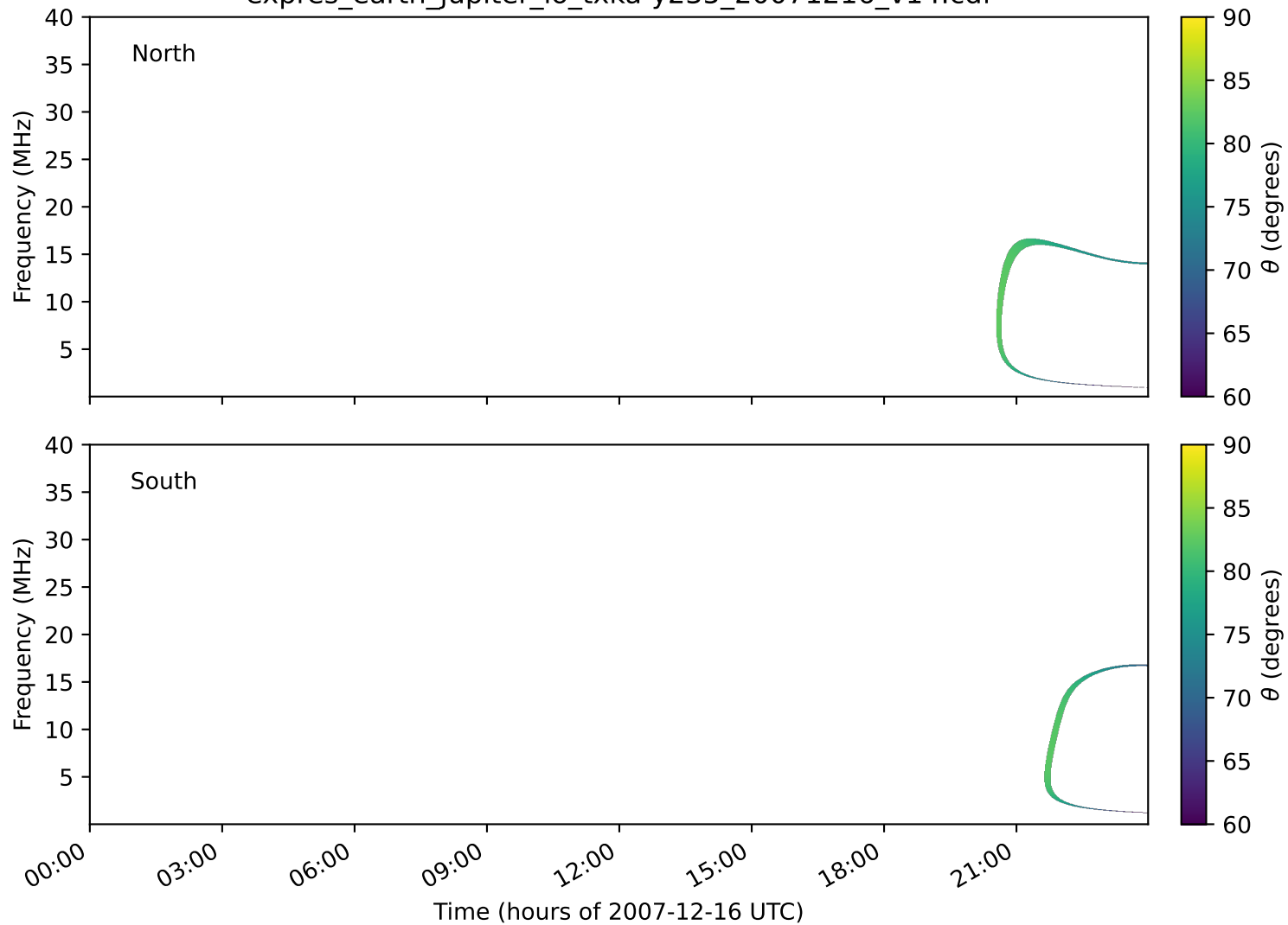
expres_earth_jupiter_io_txka-y235_20071216_v14.cdf
