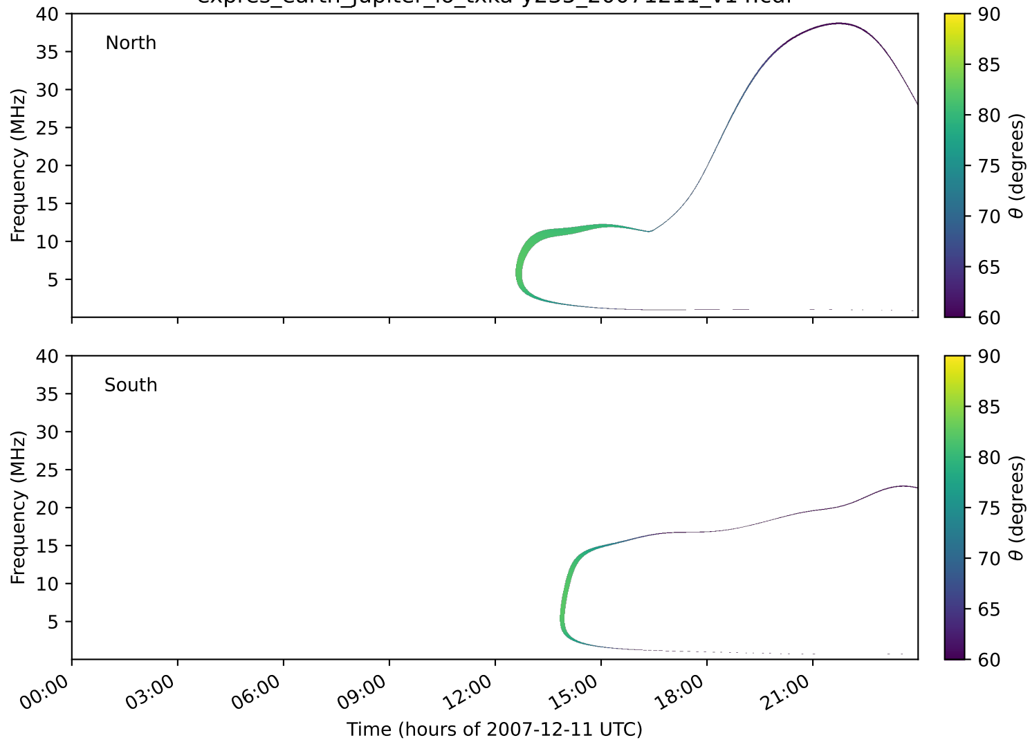
expres_earth_jupiter_io_txka-y235_20071211_v14.cdf
