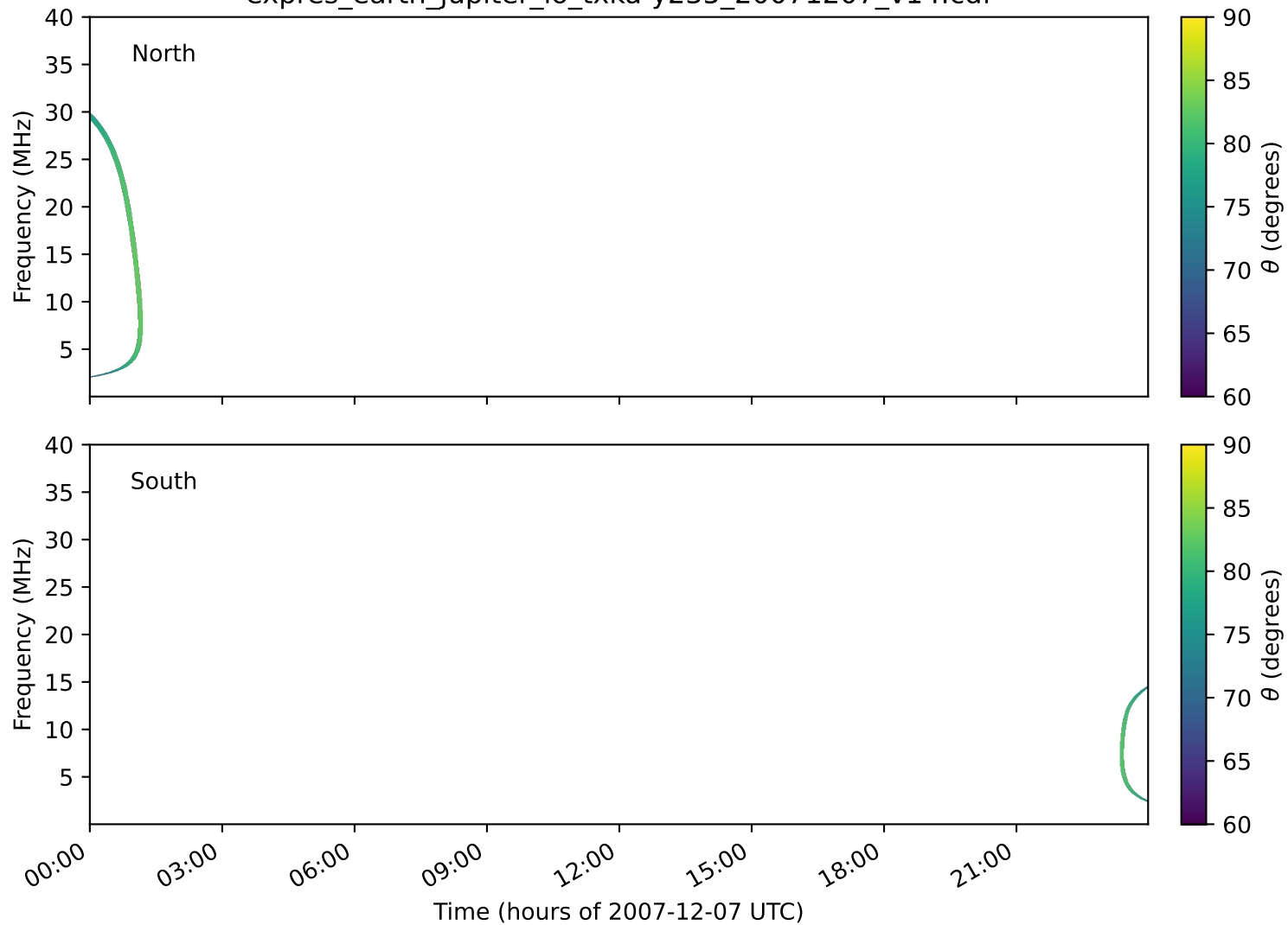
expres_earth_jupiter_io_txka-y235_20071207_v14.cdf
