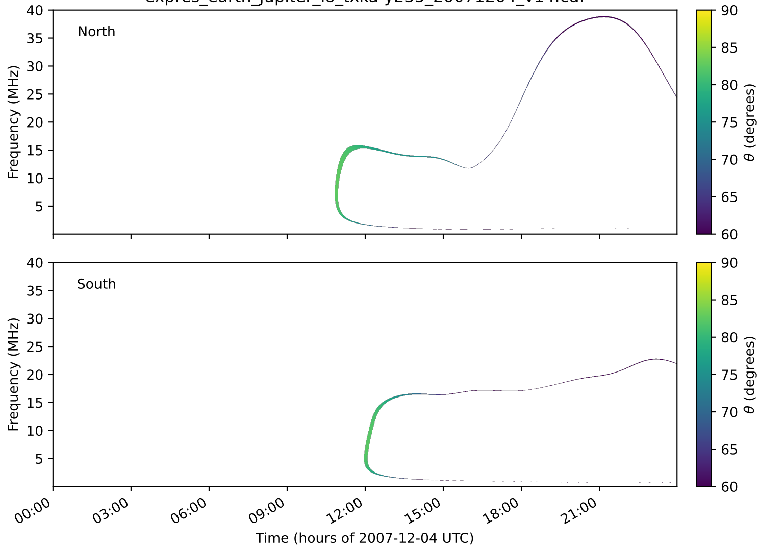
expres_earth_jupiter_io_txka-y235_20071204_v14.cdf
