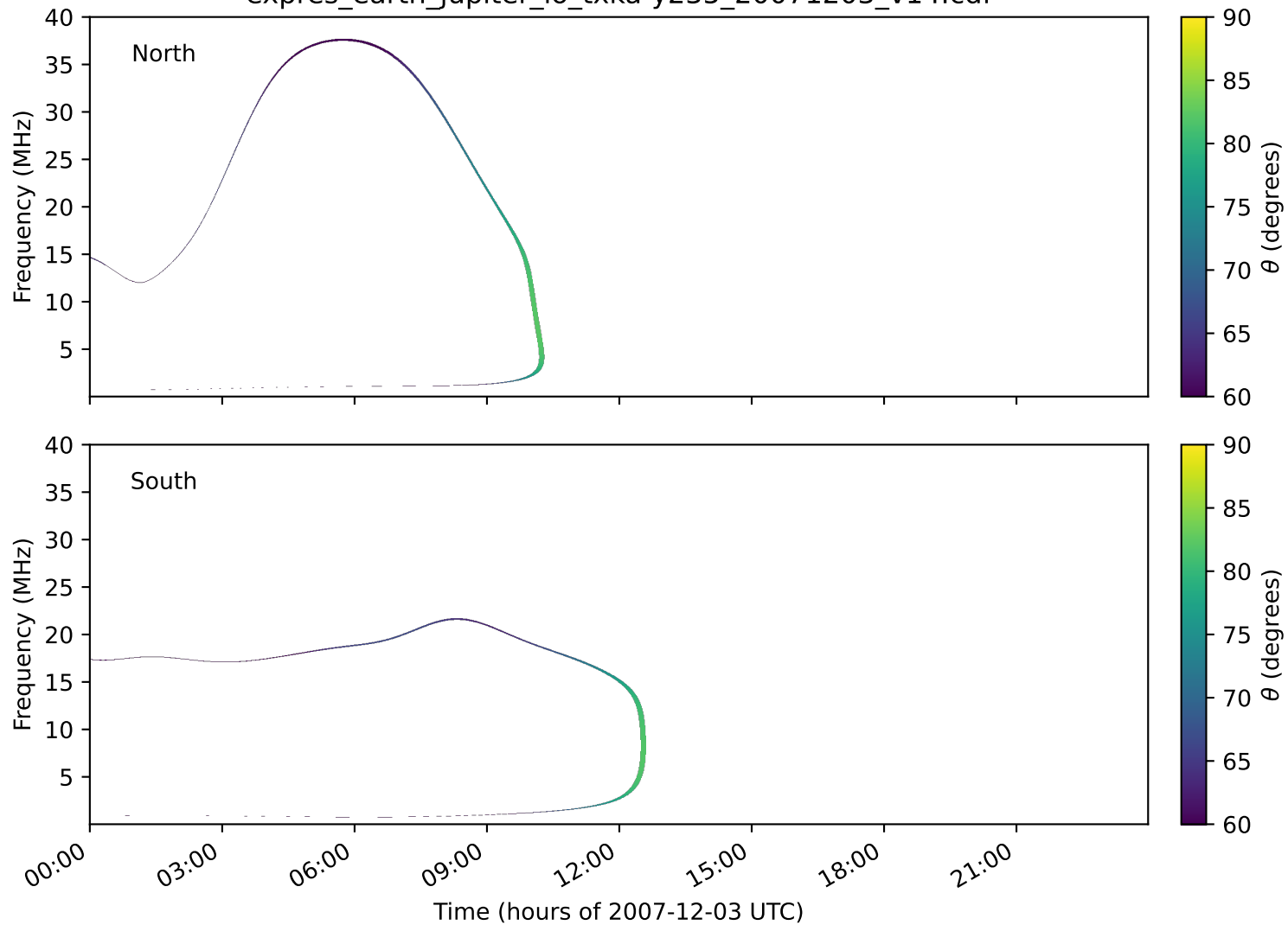
expres_earth_jupiter_io_txka-y235_20071203_v14.cdf
