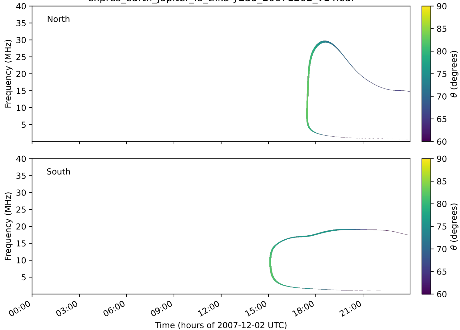
expres_earth_jupiter_io_txka-y235_20071202_v14.cdf
