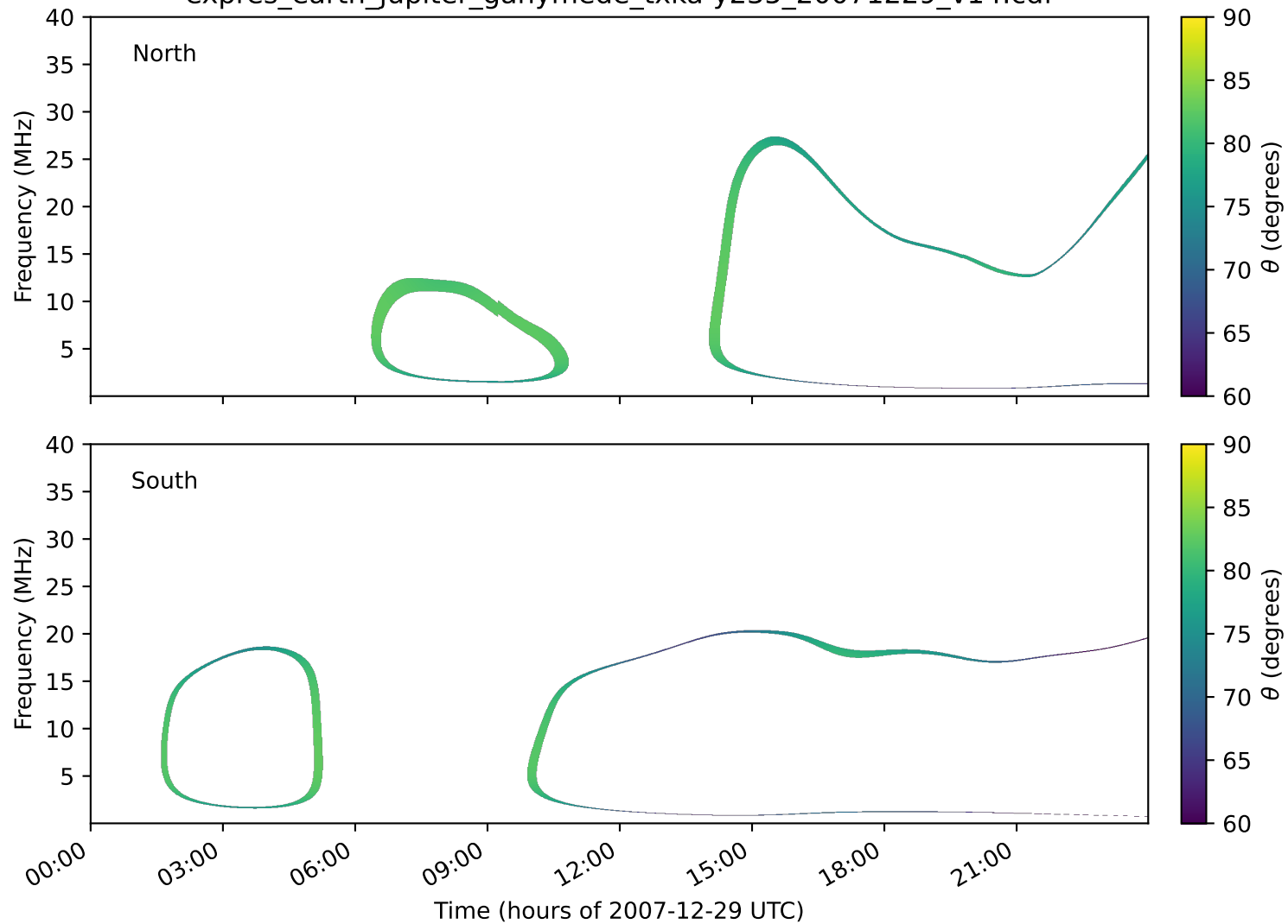
expres_earth_jupiter_ganymede_txka-y235_20071229_v14.cdf
