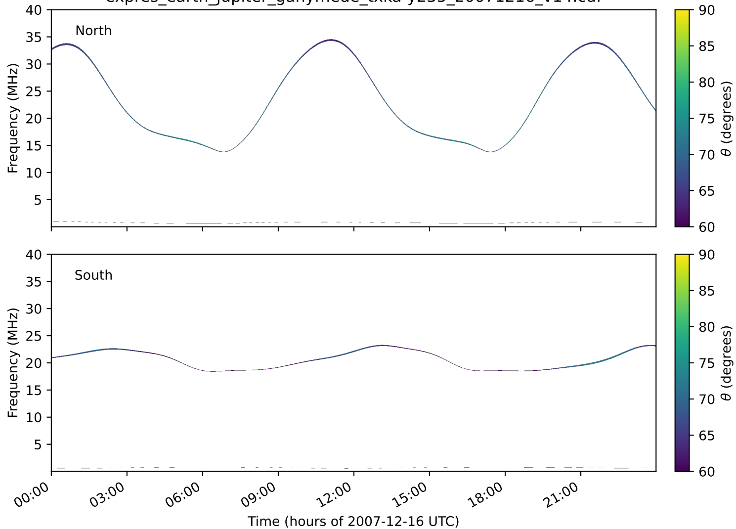
expres_earth_jupiter_ganymede_txka-y235_20071216_v14.cdf
