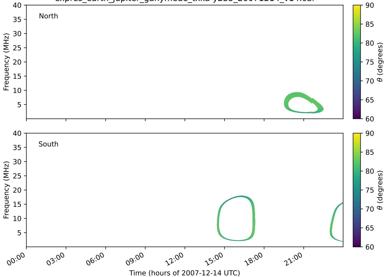
expres_earth_jupiter_ganymede_txka-y235_20071214_v14.cdf
