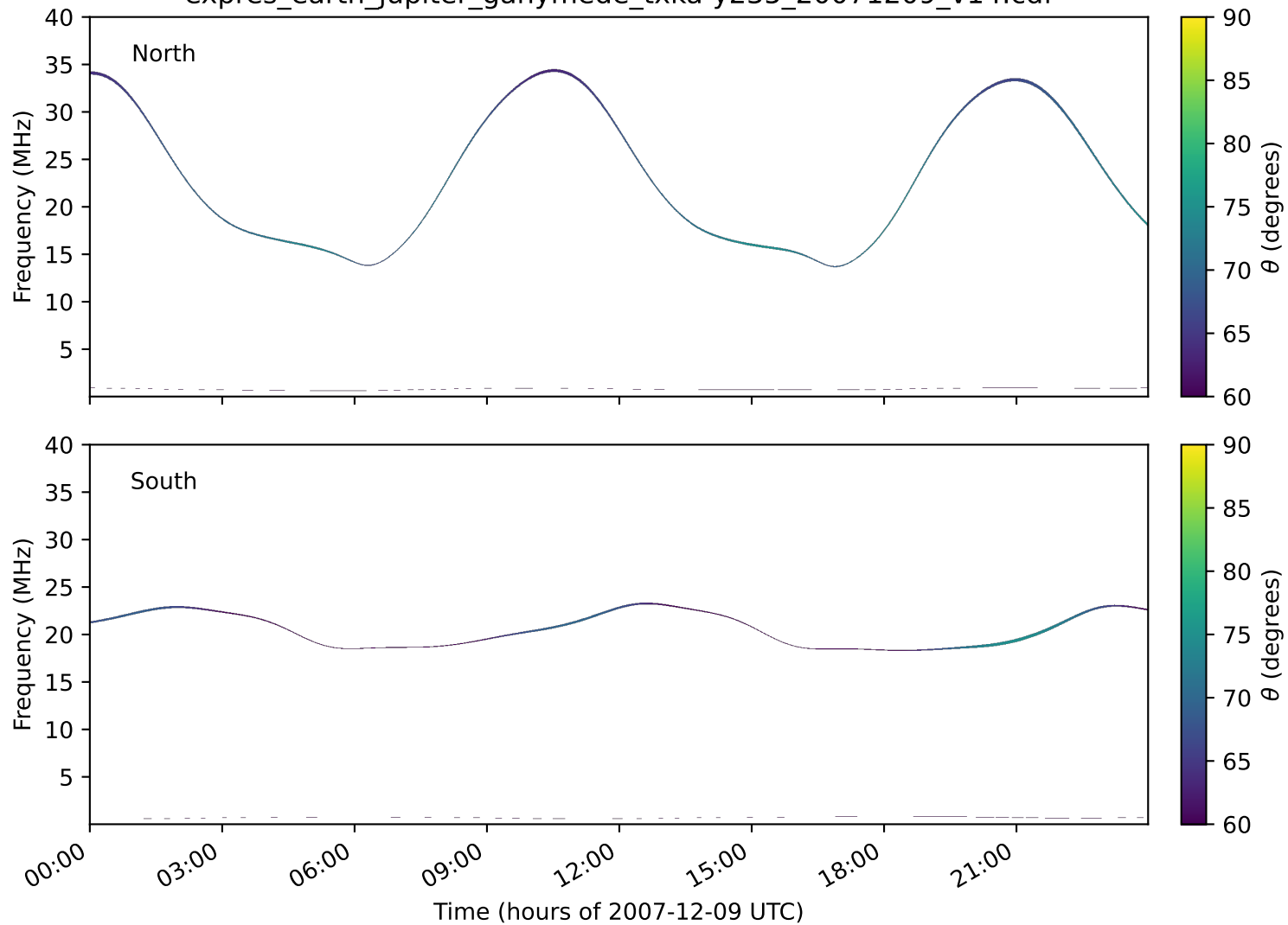
expres_earth_jupiter_ganymede_txka-y235_20071209_v14.cdf
