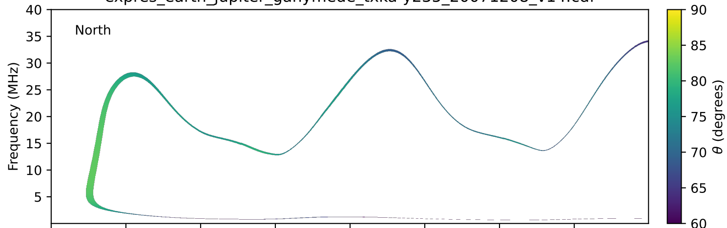
expres_earth_jupiter_ganymede_txka-y235_20071208_v14.cdf
