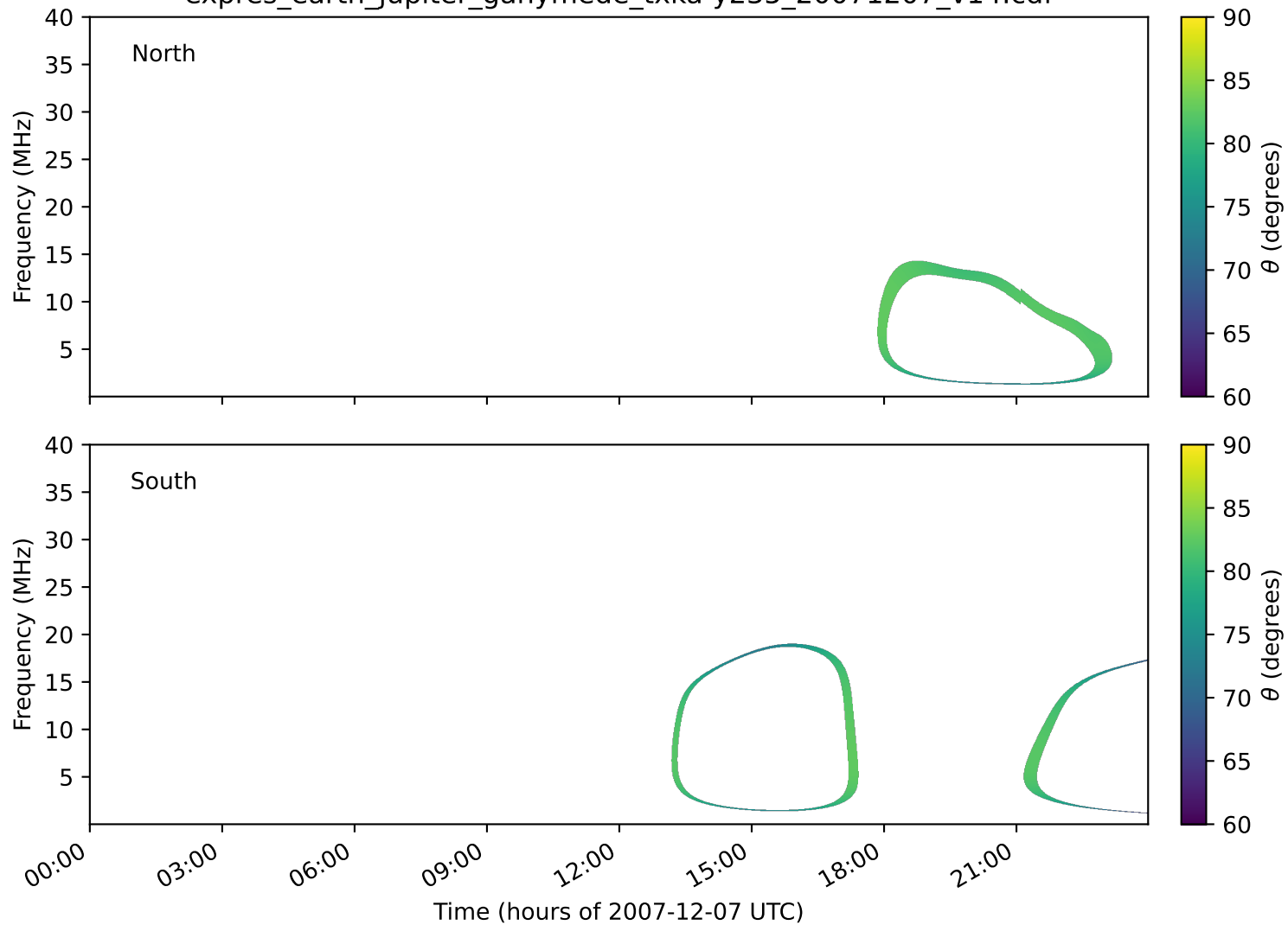
expres_earth_jupiter_ganymede_txka-y235_20071207_v14.cdf
