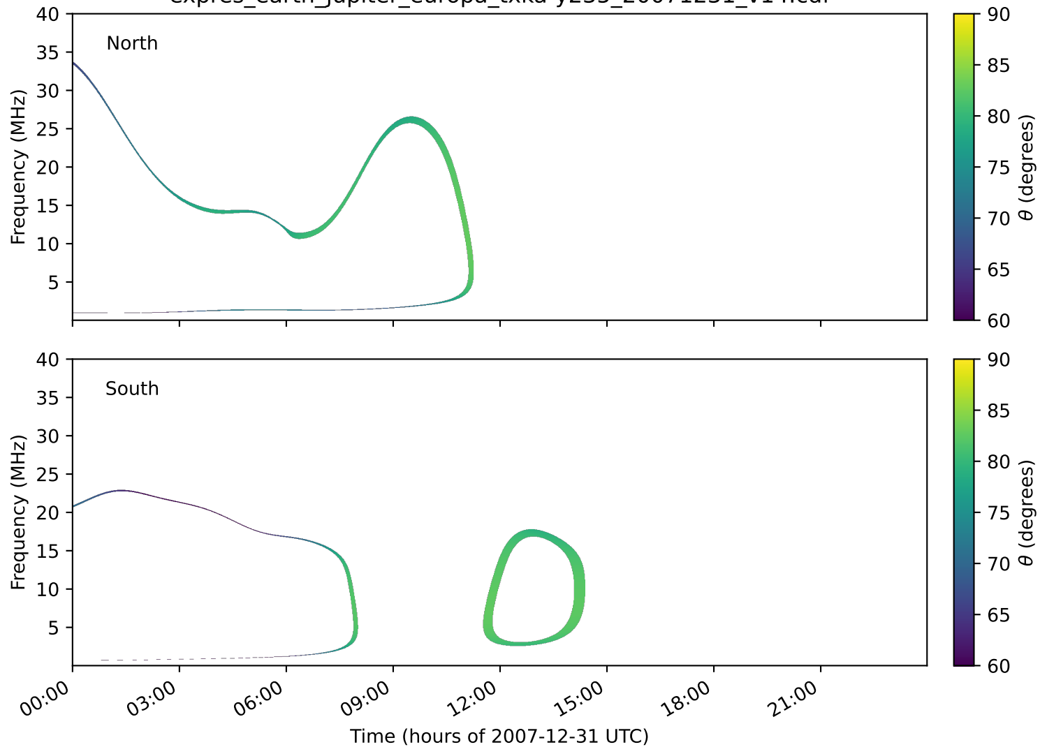
expres_earth_jupiter_europa_txka-y235_20071231_v14.cdf
