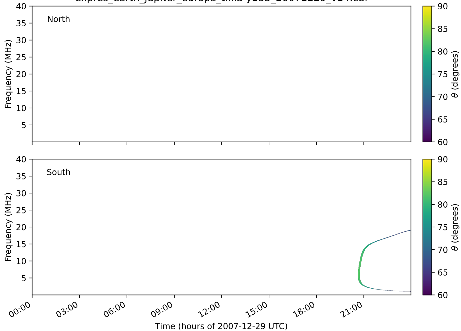
expres_earth_jupiter_europa_txka-y235_20071229_v14.cdf
