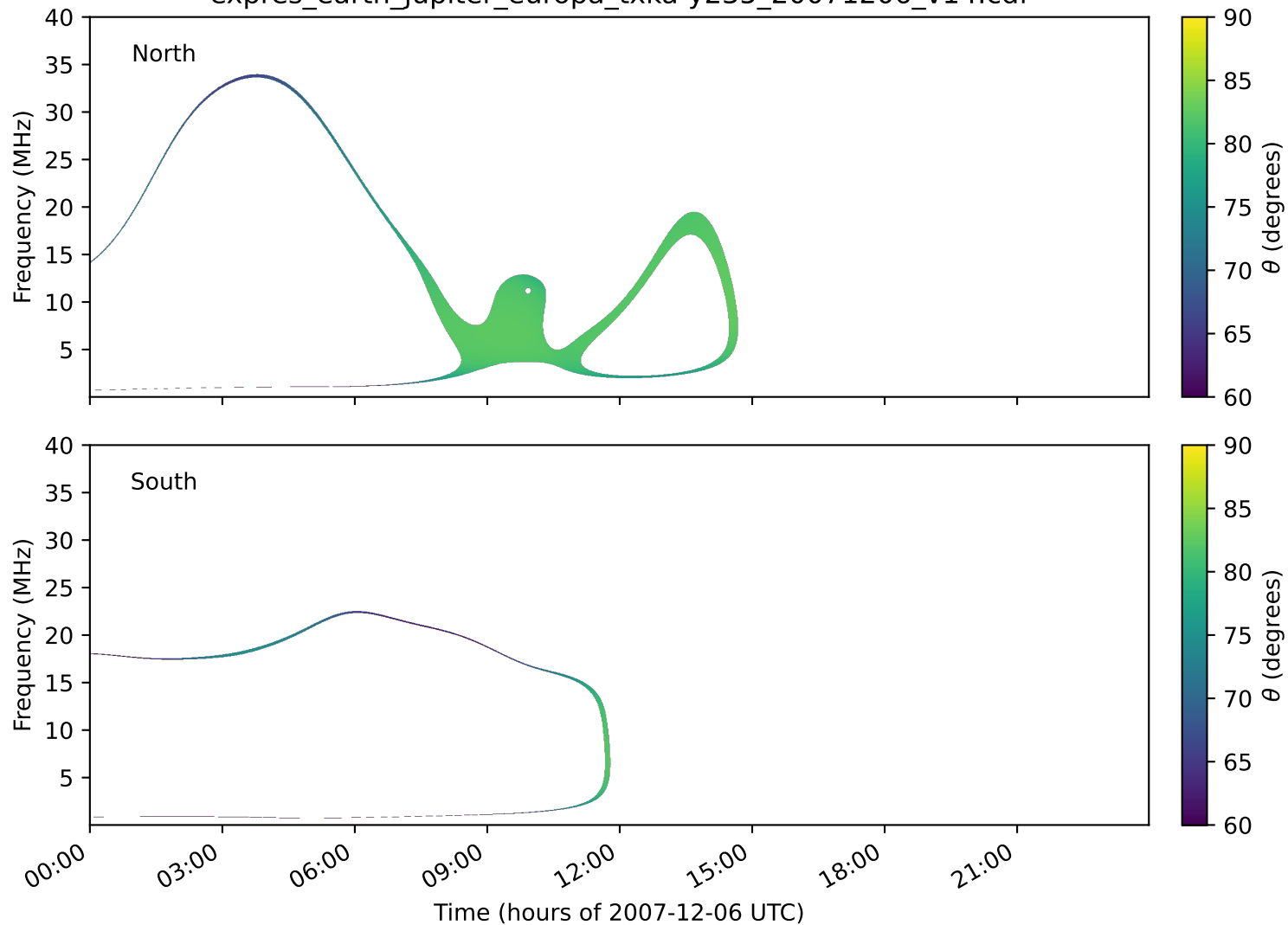
expres_earth_jupiter_europa_txka-y235_20071206_v14.cdf
