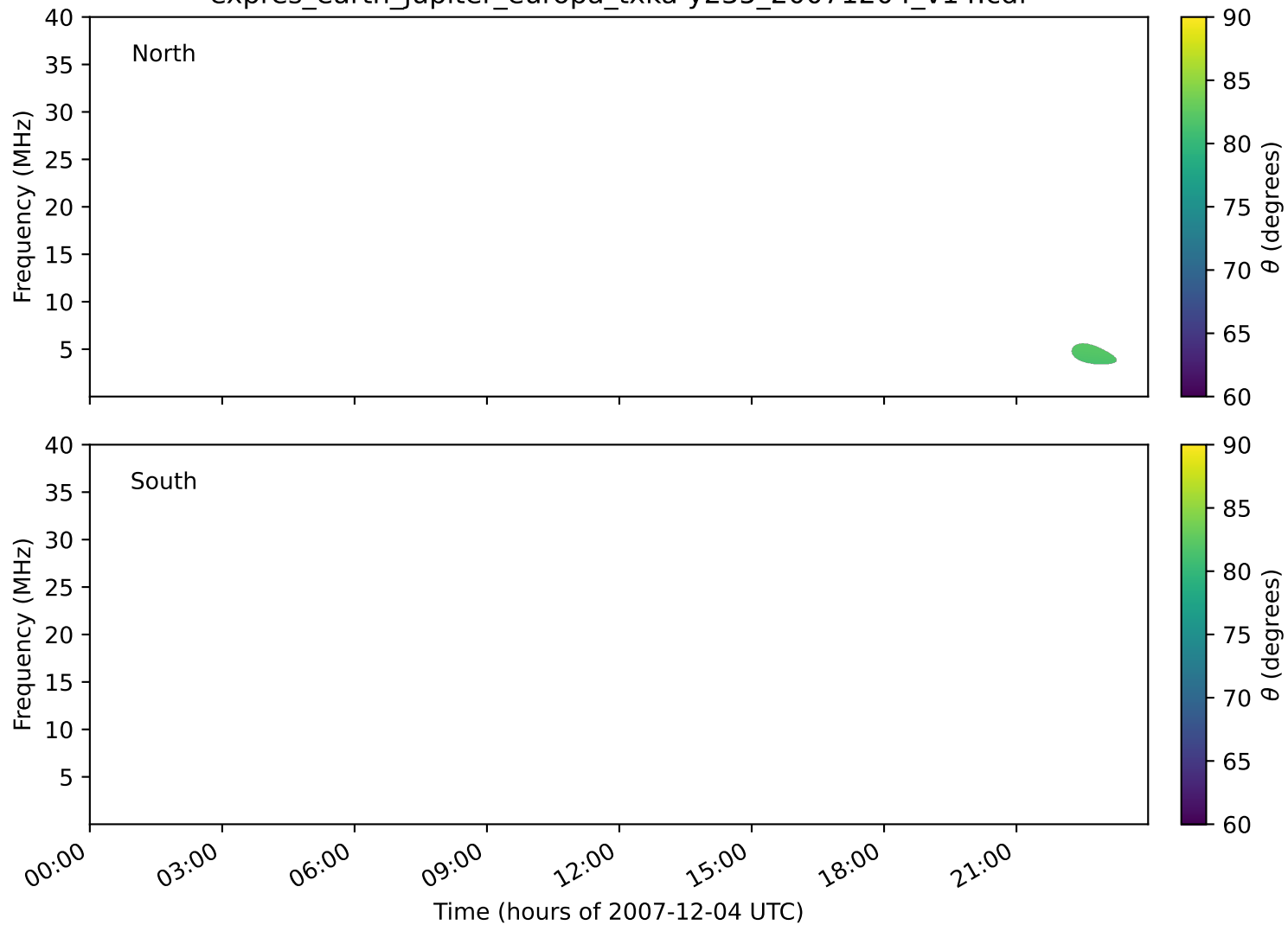
expres_earth_jupiter_europa_txka-y235_20071204_v14.cdf
