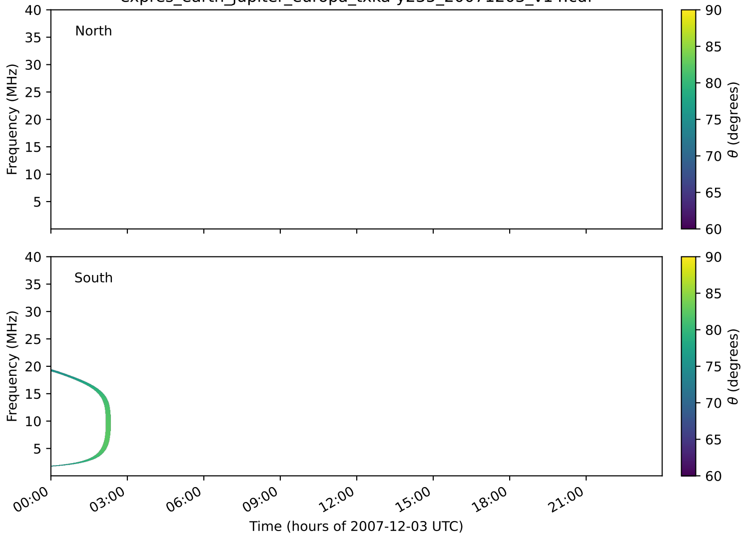
expres_earth_jupiter_europa_txka-y235_20071203_v14.cdf
