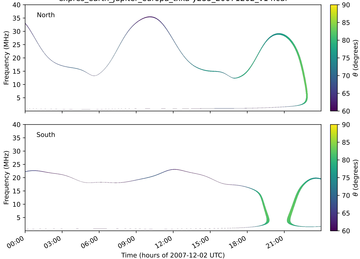
expres_earth_jupiter_europa_txka-y235_20071202_v14.cdf
