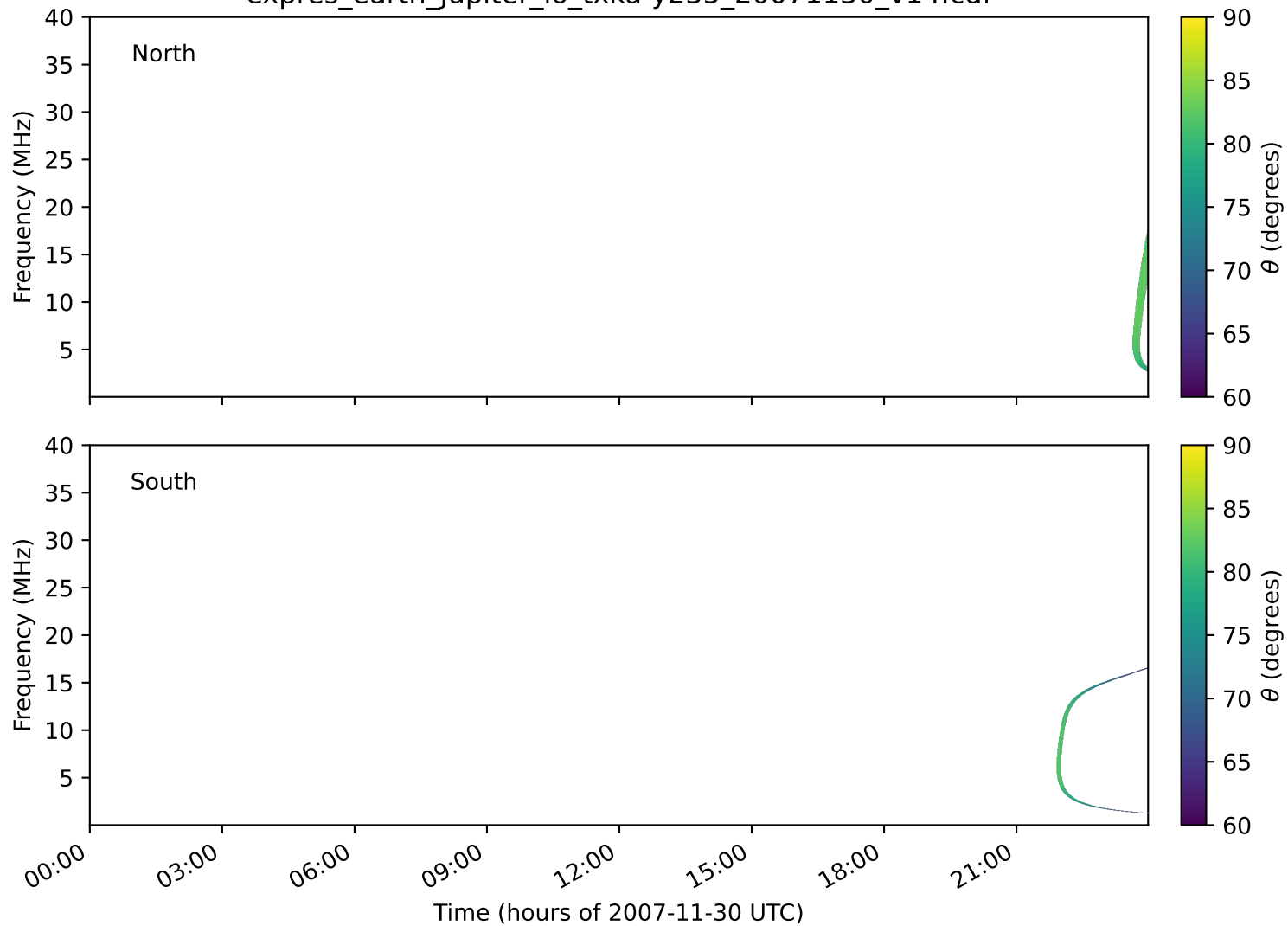
expres_earth_jupiter_io_txka-y235_20071130_v14.cdf
