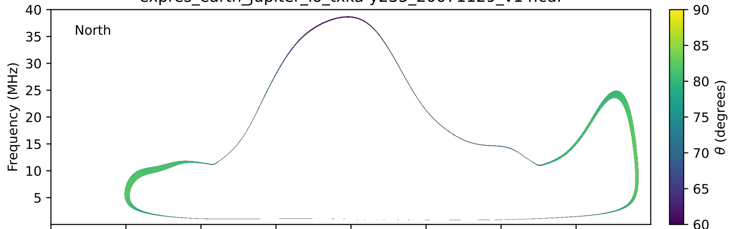
expres_earth_jupiter_io_txka-y235_20071129_v14.cdf
