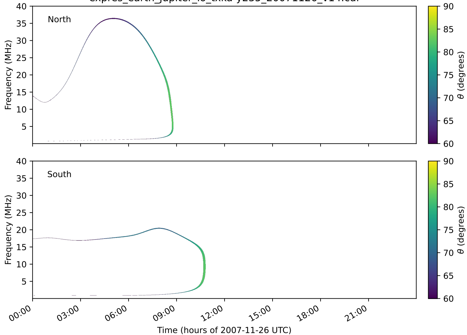
expres_earth_jupiter_io_txka-y235_20071126_v14.cdf
