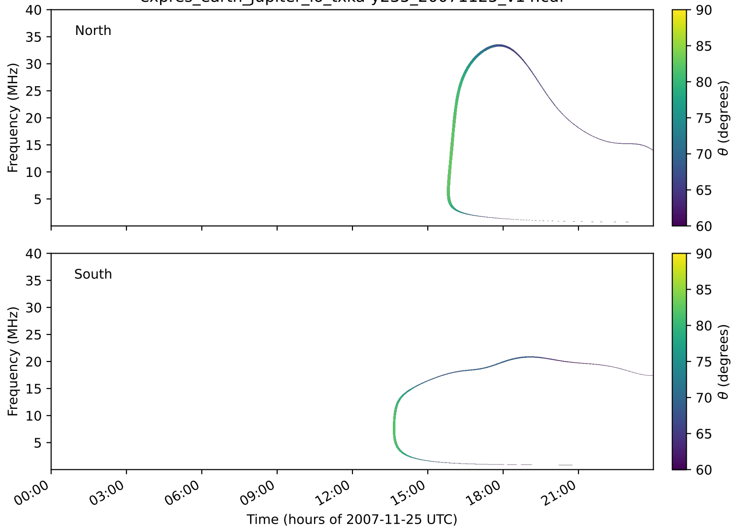
expres_earth_jupiter_io_txka-y235_20071125_v14.cdf
