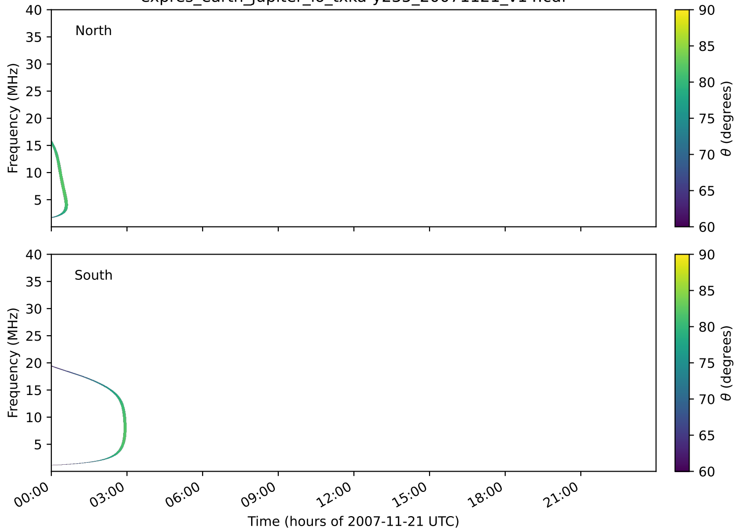
expres_earth_jupiter_io_txka-y235_20071121_v14.cdf
