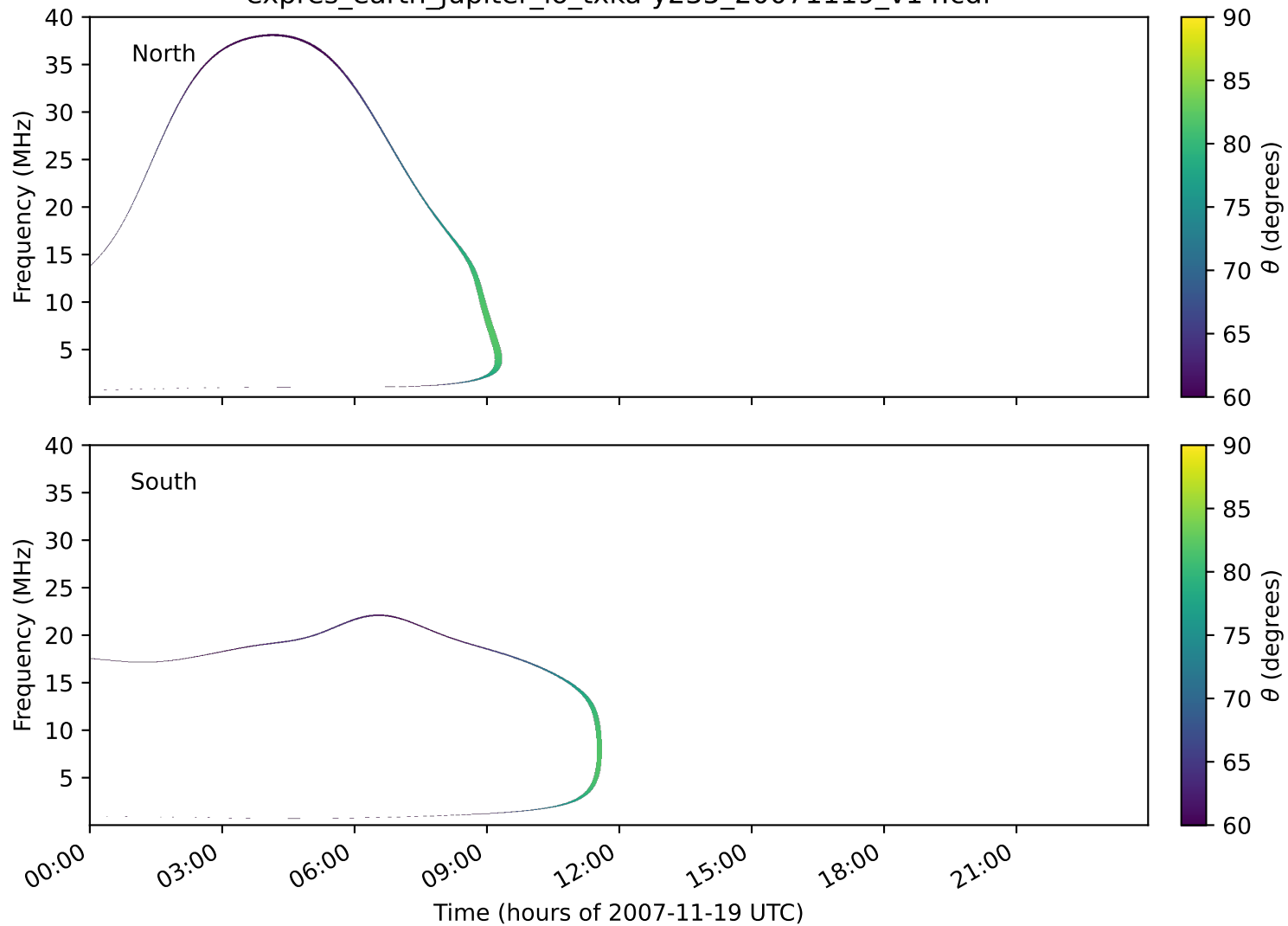
expres_earth_jupiter_io_txka-y235_20071119_v14.cdf
