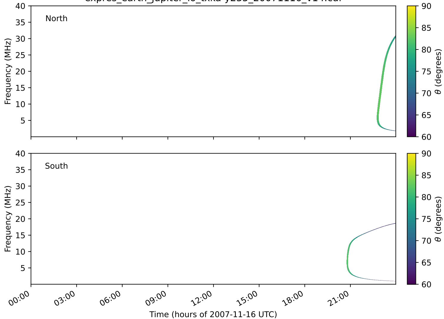
expres_earth_jupiter_io_txka-y235_20071116_v14.cdf
