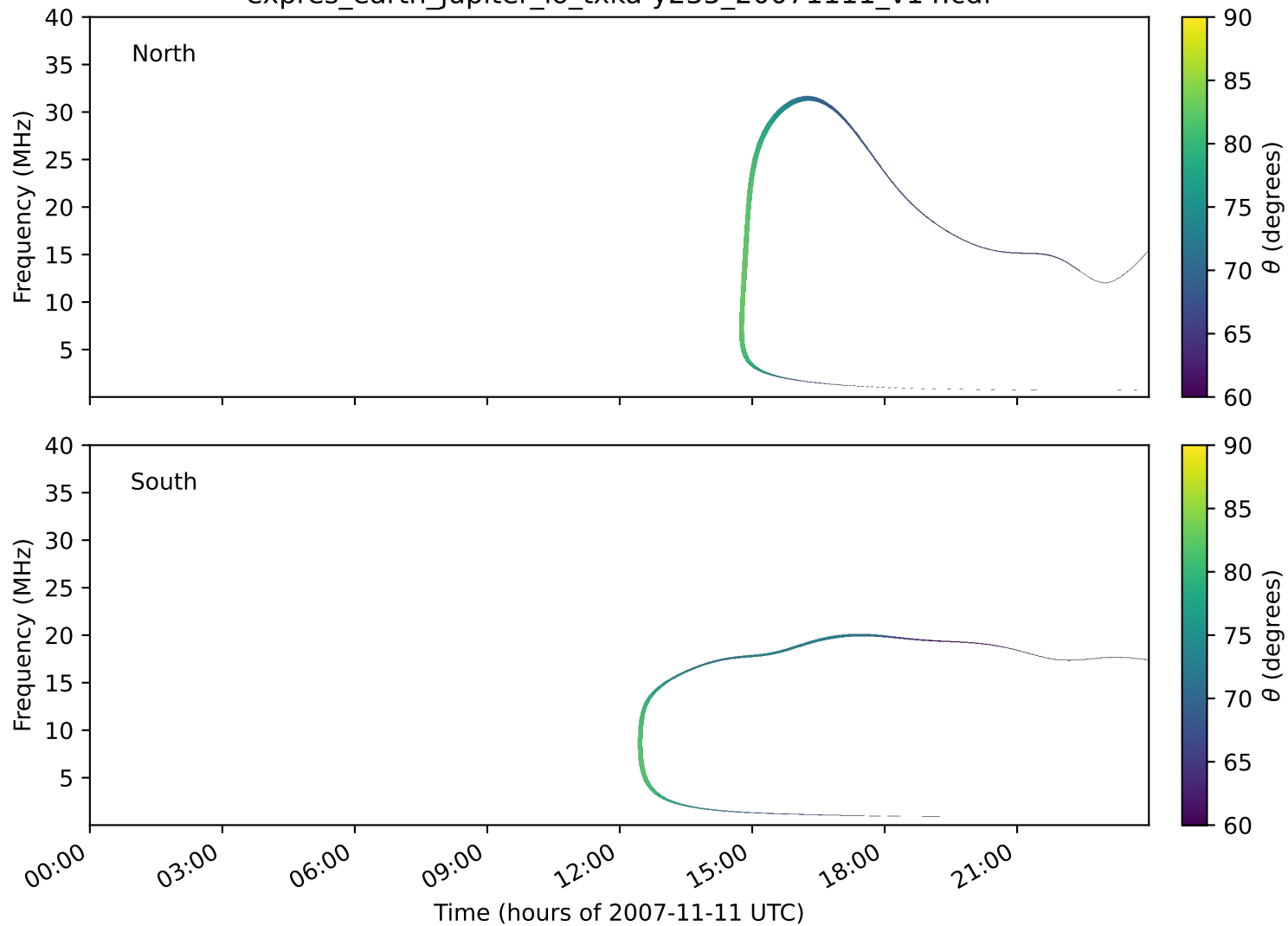
expres_earth_jupiter_io_txka-y235_20071111_v14.cdf
