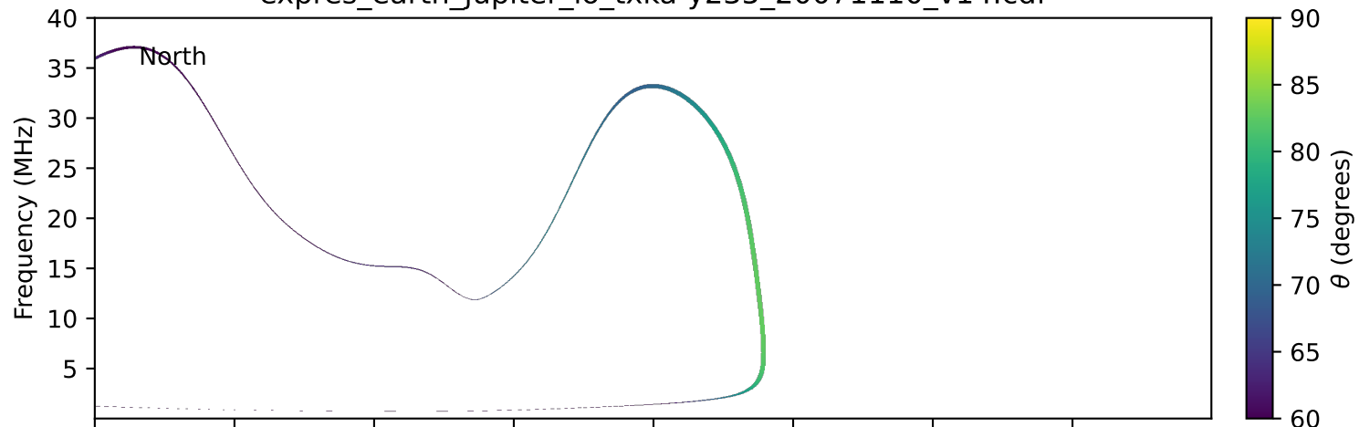
expres_earth_jupiter_io_txka-y235_20071110_v14.cdf
