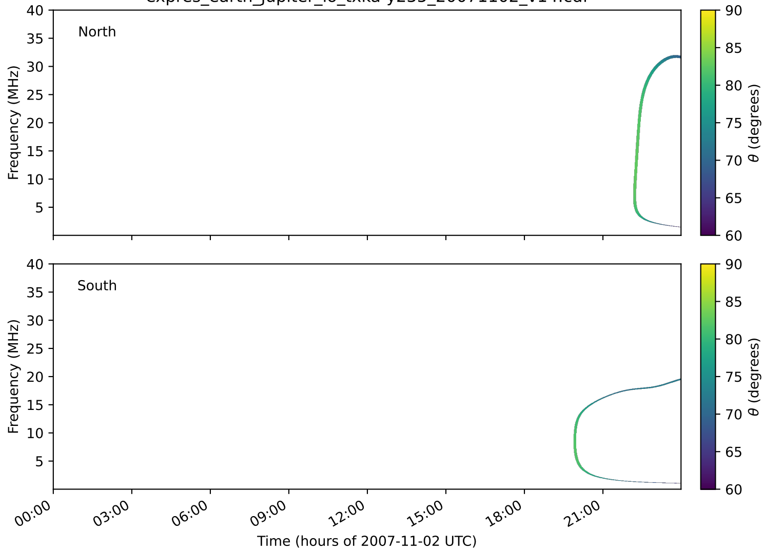
expres_earth_jupiter_io_txka-y235_20071102_v14.cdf
