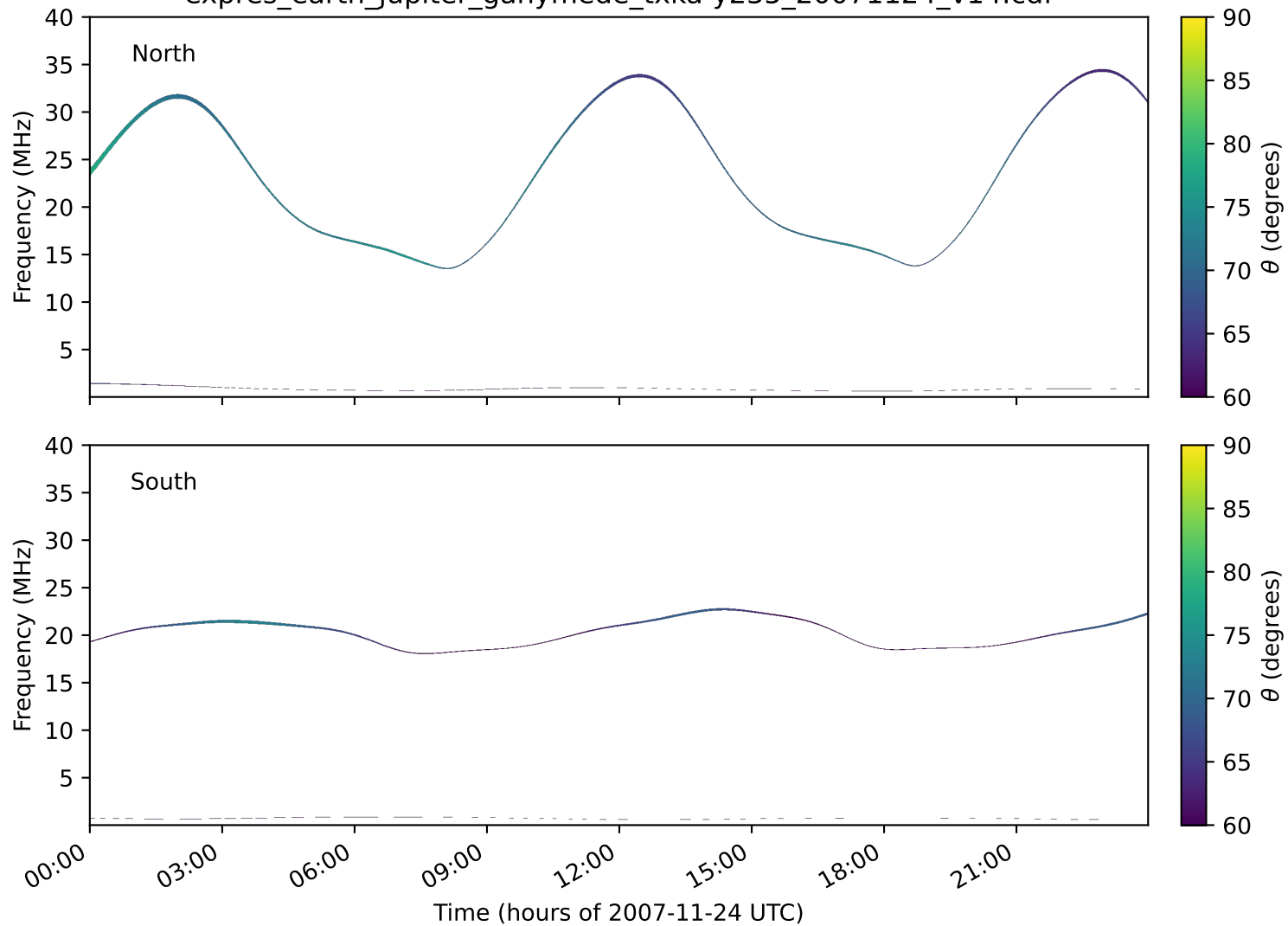
expres_earth_jupiter_ganymede_txka-y235_20071124_v14.cdf
