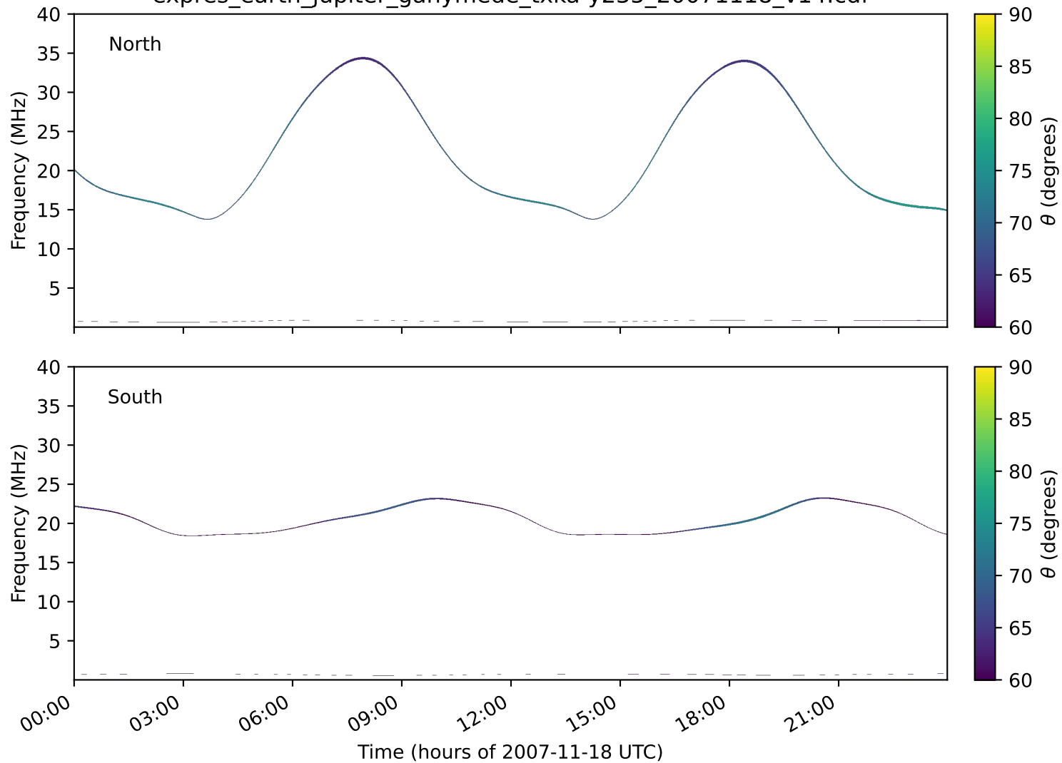
expres_earth_jupiter_ganymede_txka-y235_20071118_v14.cdf
