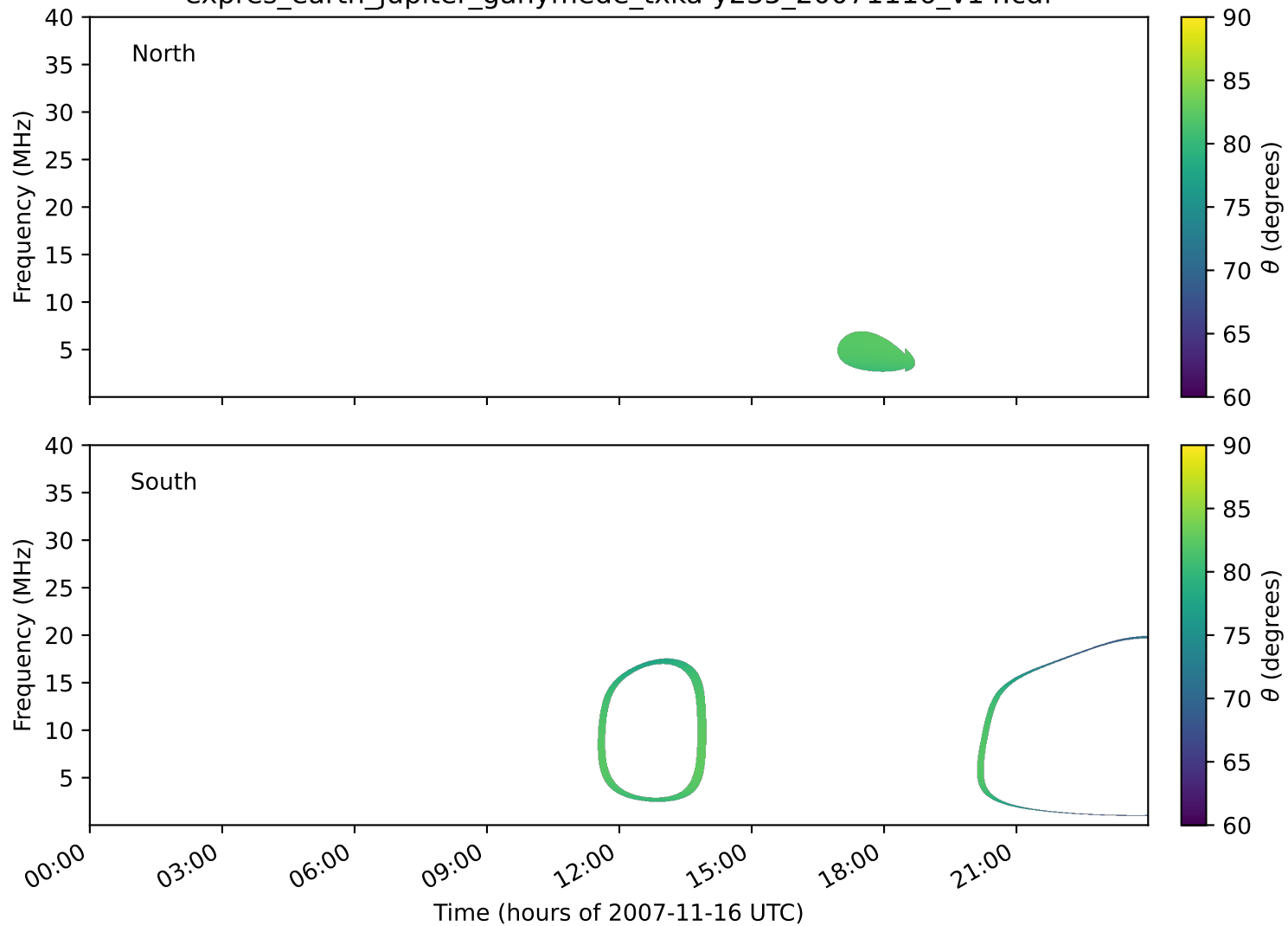
expres_earth_jupiter_ganymede_txka-y235_20071116_v14.cdf
