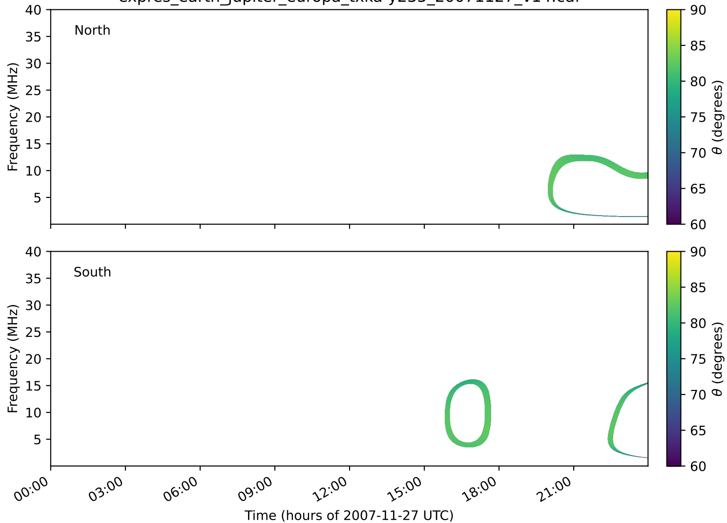
expres_earth_jupiter_europa_txka-y235_20071127_v14.cdf
