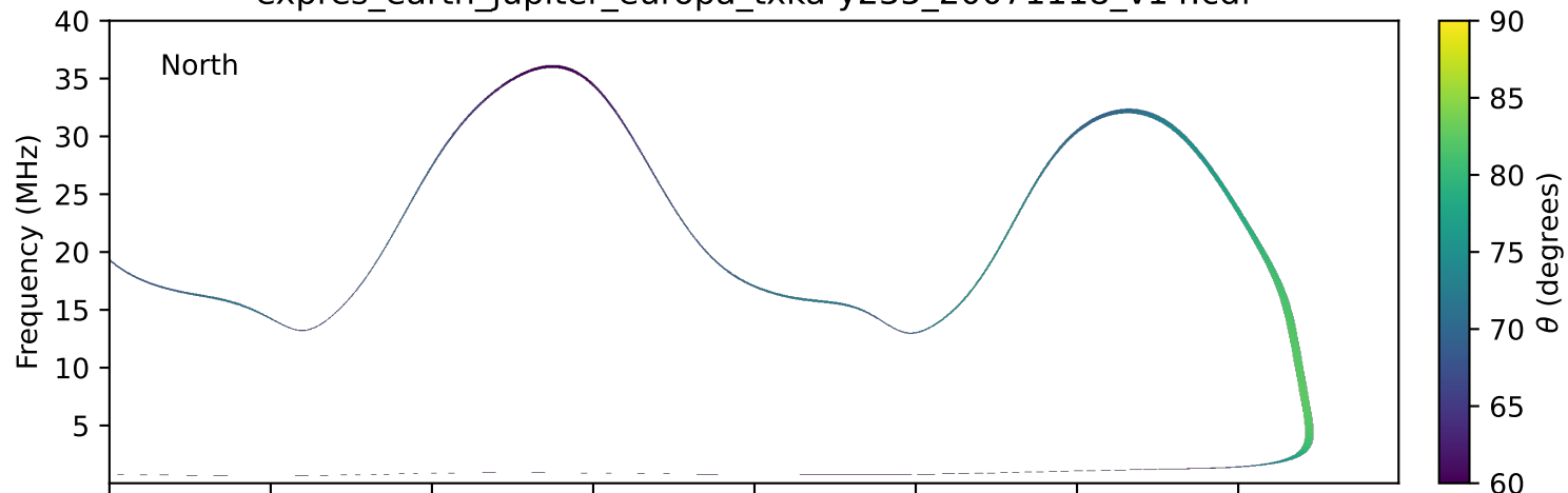
expres_earth_jupiter_europa_txka-y235_20071118_v14.cdf
